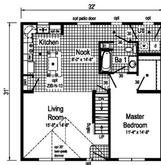
Main Floor
