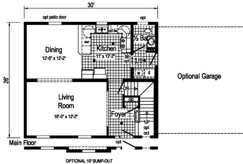
6M3001-N 2630 Approx. 1560 Sq. Ft.
